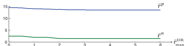
Fig. 3. Optimal thresholds for primary and ancillary service
